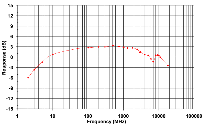
FL7218 Typical Uncalibrated Frequency Response
