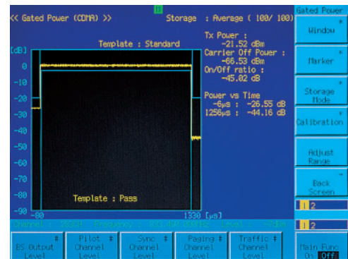
Gated output power measurement
