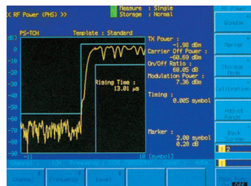
Example of burst rise characteristics (PHS)
