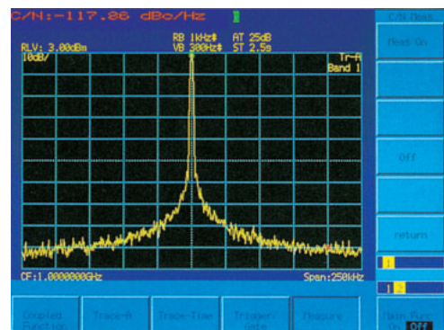
C/N measurement
