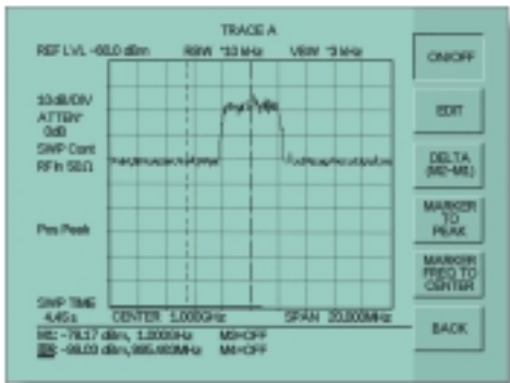
Preamplifier Off
